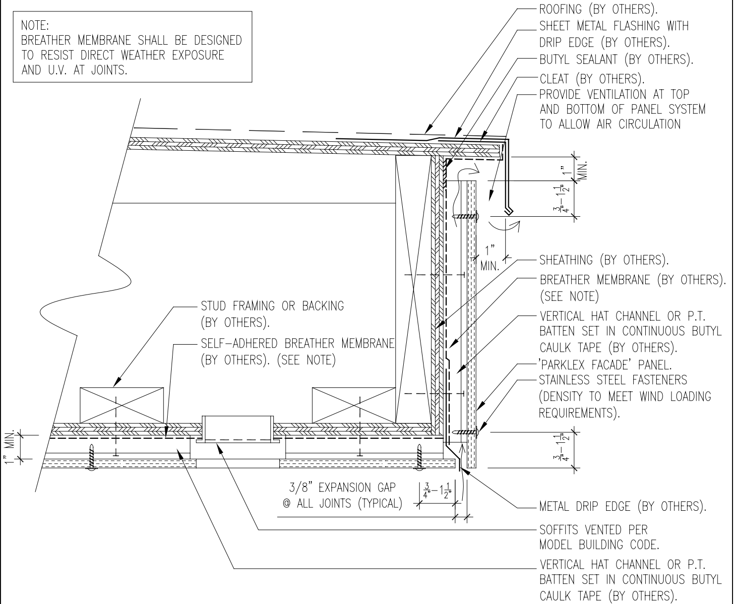
PARKLEX FACADE OUTER EAVE DETAIL
