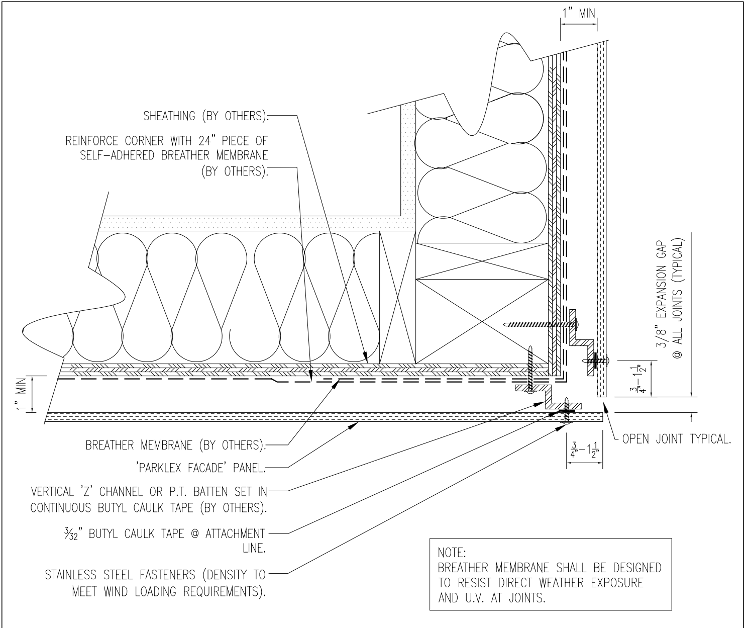
PARKLEX FACADE OUTER CORNER DETAIL
