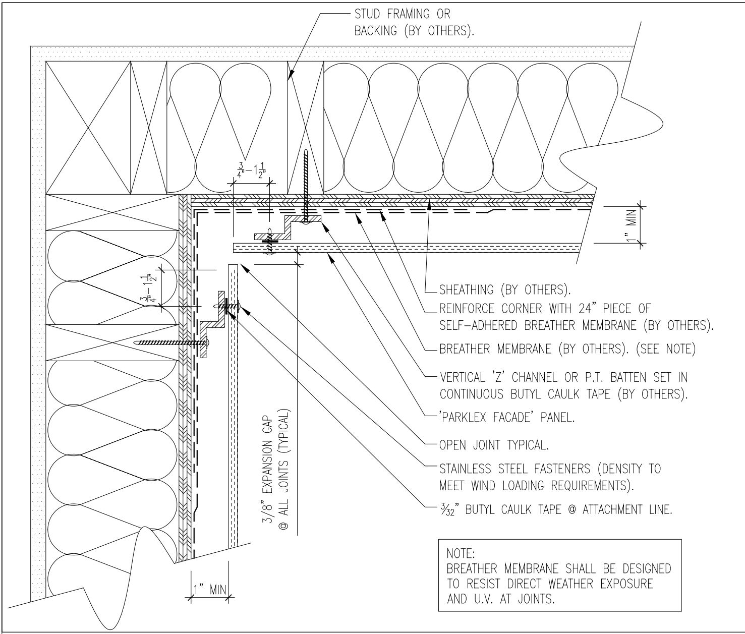
PARKLEX FACADE INNER CORNER DETAIL
