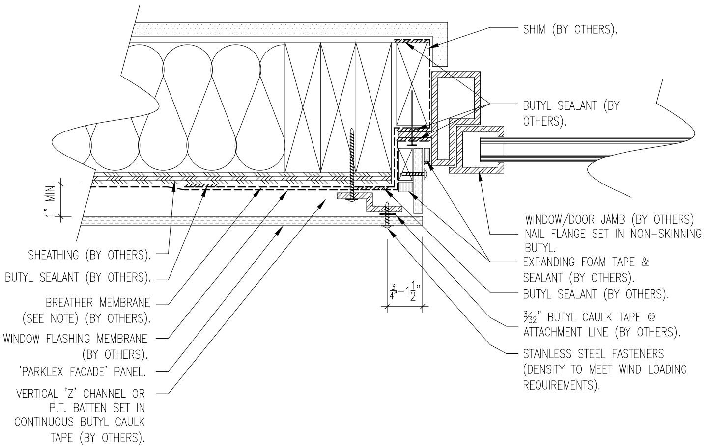
WINDOW DETAIL 7 FLANGED WINDOW
