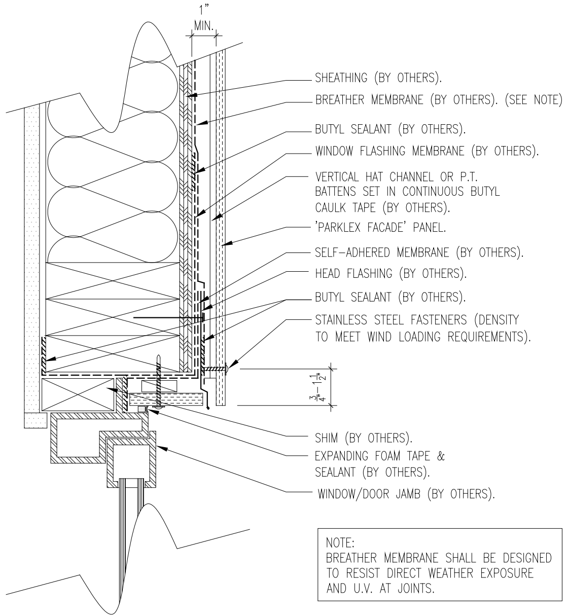
PARKLEX FACADE WINDOW HEAD DETAIL
