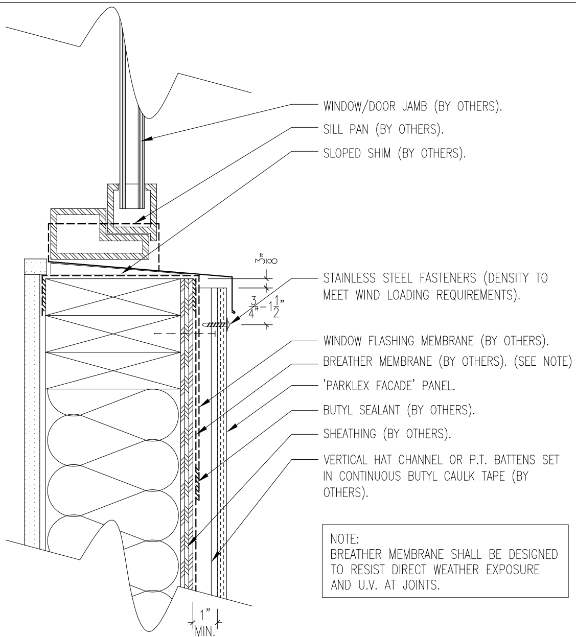
PARKLEX FACADE WINDOW SILL DETAIL
